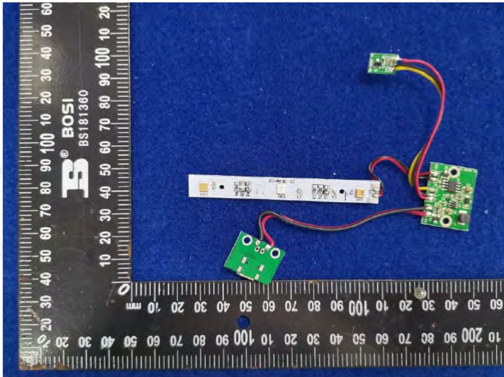
Photo 5: PCB view
